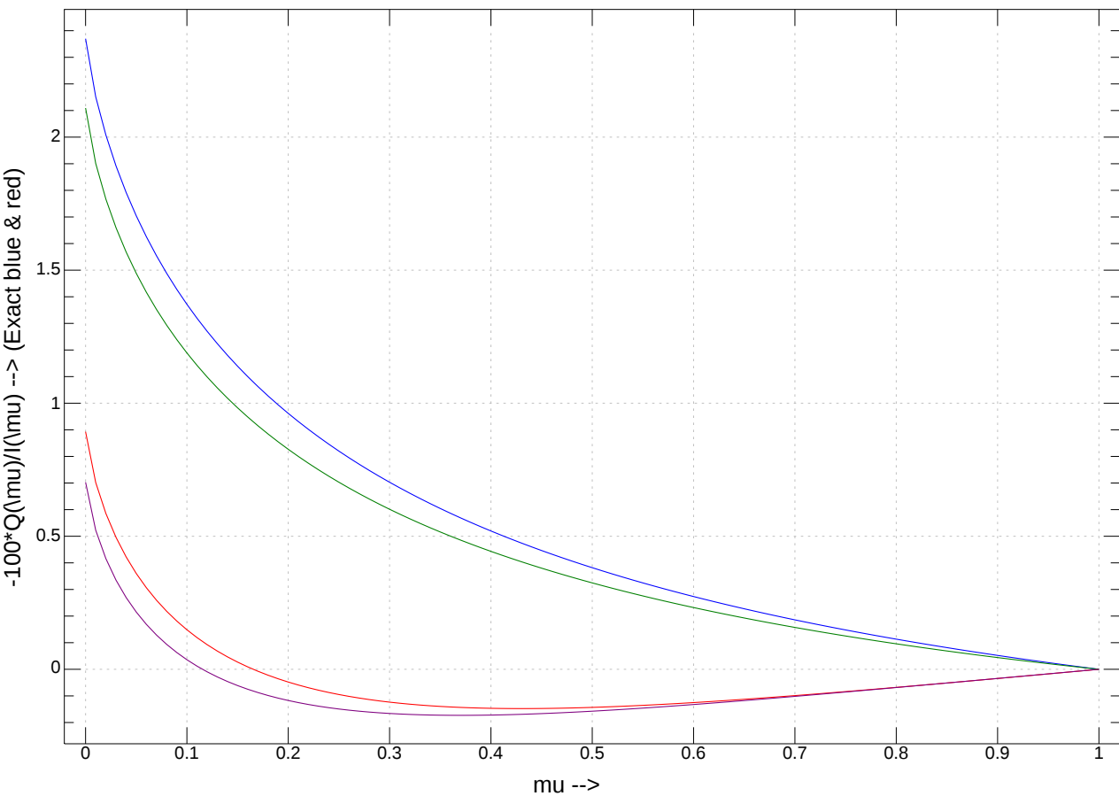
Percent polarization for Exact & Approx B=a+b*tau for a=1,b=0.5,1.5 and Sigma=0.3
