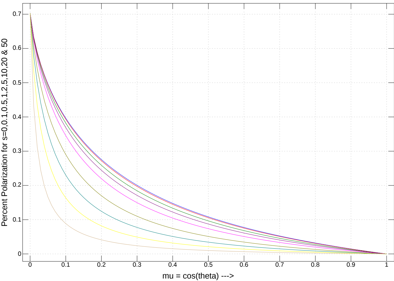
Polarization vs. \mu for a=1, b=1.5, S_0=0.1 & \exp(-s \cdot \tau)
