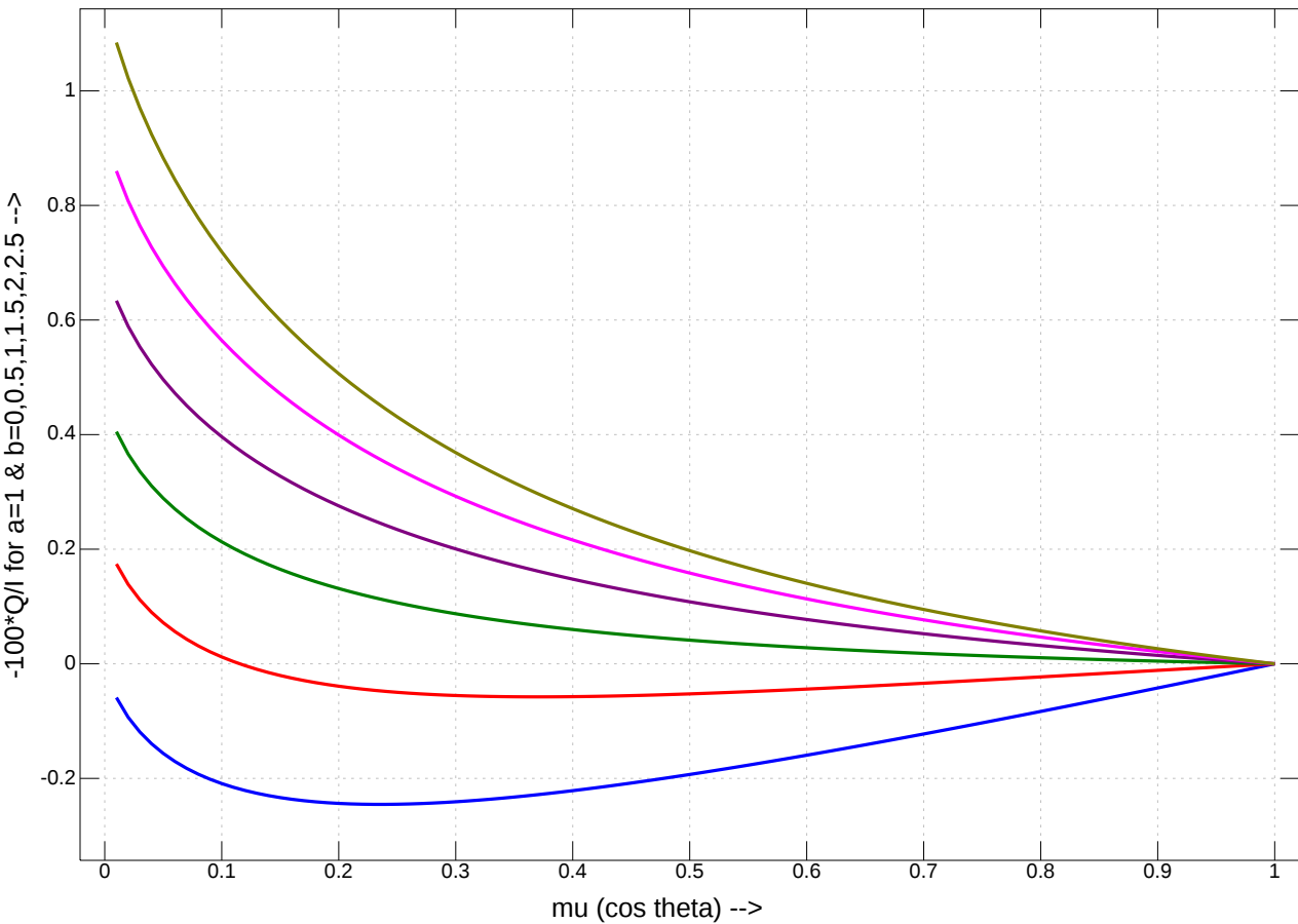
Polarization vs. \mu for s(\tau) = a+b\tau
