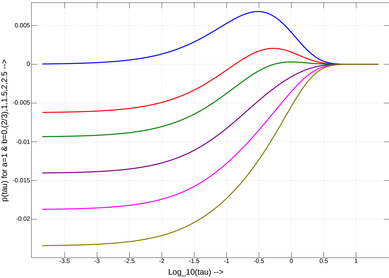
Polarization source term p(\tau) for s(\tau) = a + b \cdot \tau
