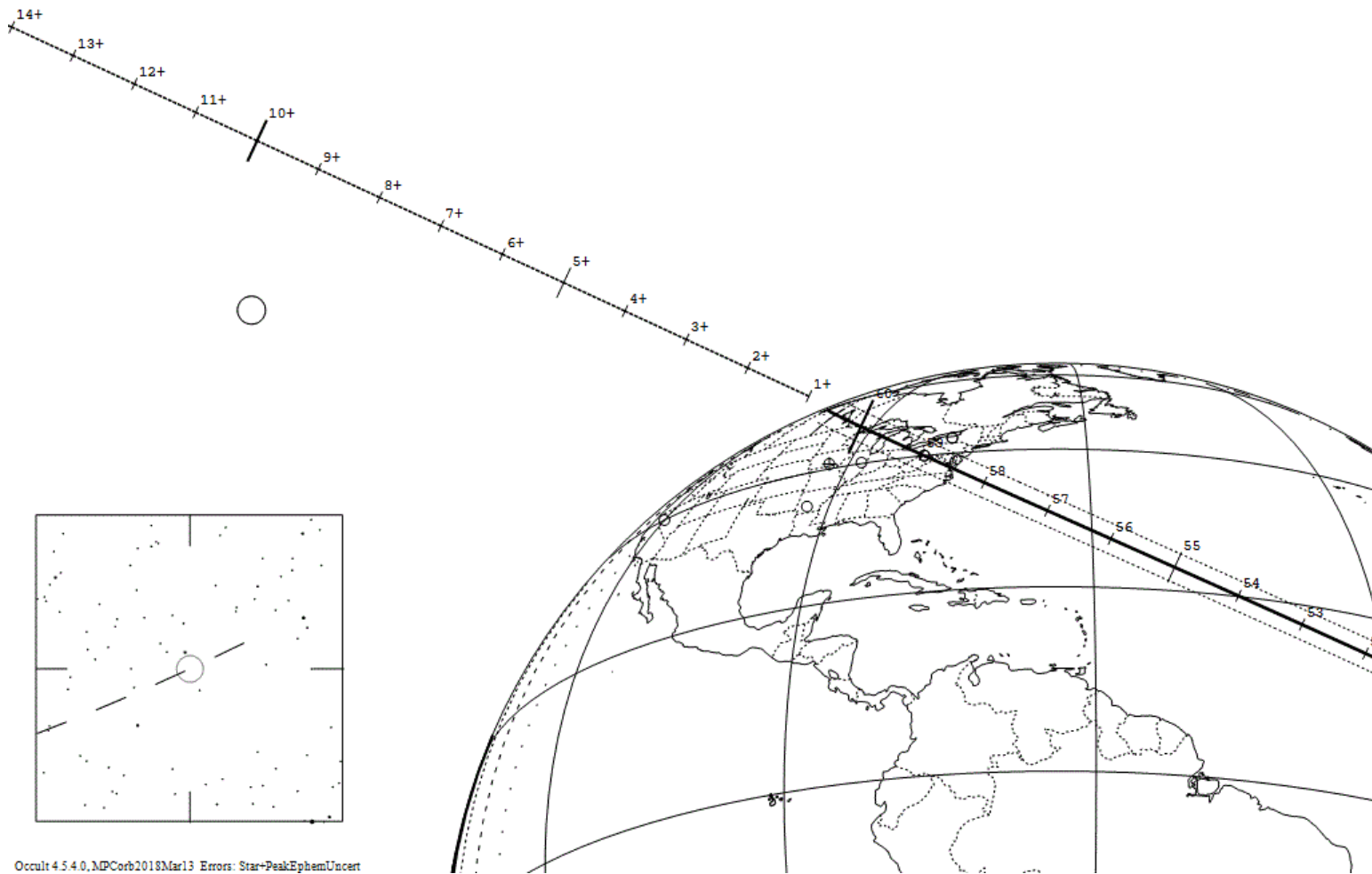
Occult 4.5.4.0, MPCorb2018Mar13 Errors: Star+PeakEphemUncert
